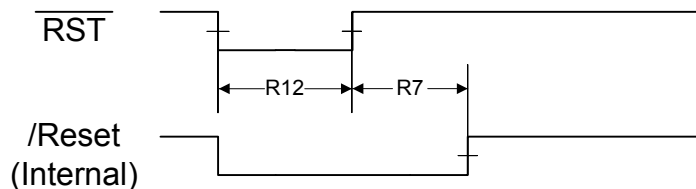
Figure 27-5. Power-On Reset Timing
