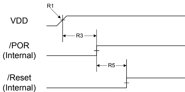
Figure 27-5. Power-On Reset Timing
